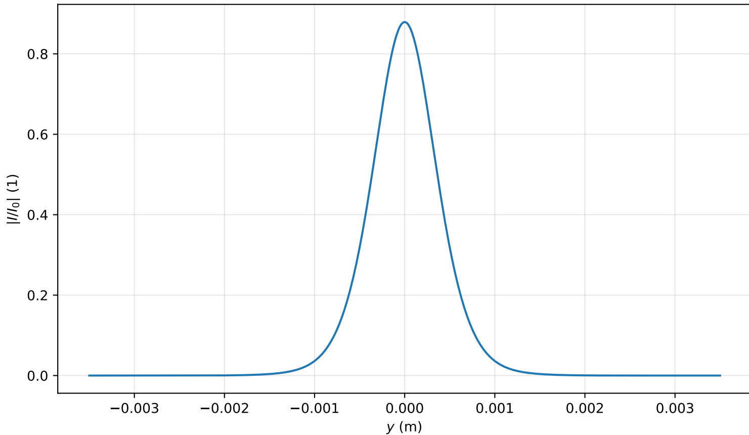
Intensity profile I(x=0, y, z=2.229)/I_0 , P_{in}=0.6P_{cr} , artificial time
